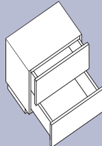
D95CP Filing drawer H550 x W600 x D450
