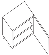
D110CM(left) D111CM(right) Single door H635 x W600 x D600
