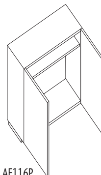
AE116P Wardrobe H1800 x W1000 x D600
